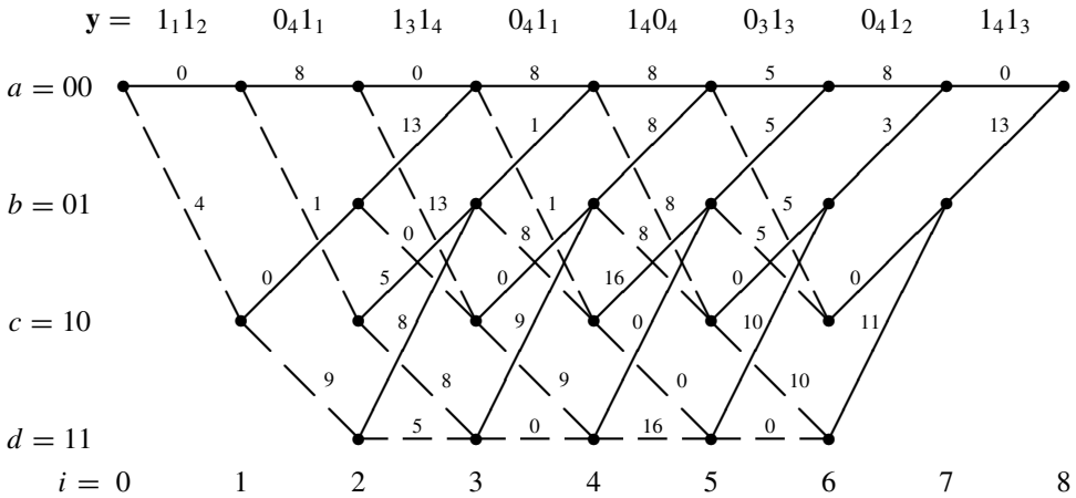
Figure 15.4 Edge weights for the Soft Decision Viterbi Algorithm.
