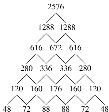
Figure 8.4 Pascal triangle of a 5-(24, 12, 48) design.
