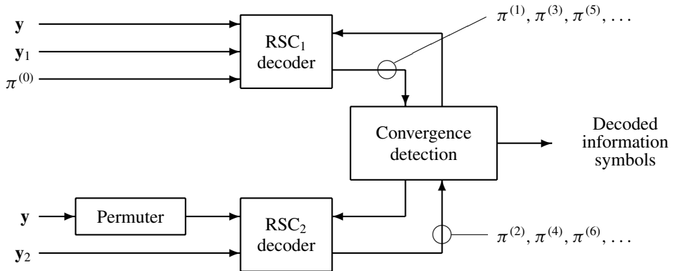
Figure 15.14 Turbo decoder.
