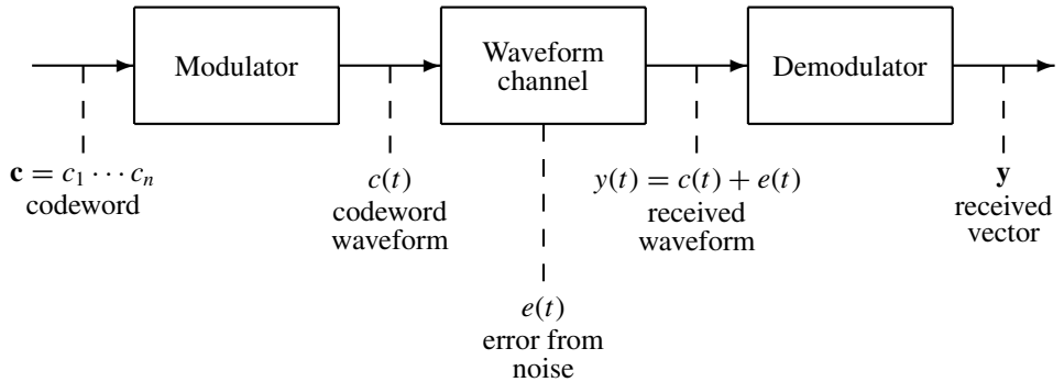
Figure 15.1 Modulated communication channel.
